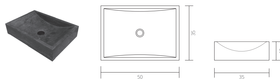
Top 5. Hardsteen rechthoek 50 x 35 x 12 cm Top 5. Blue stone rectangle 50 x 35 x 12 cm
